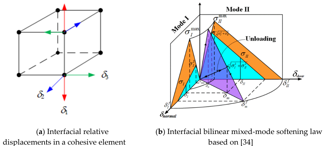
Figure 4. Cohesive zone.
